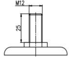
Threaded Stem
