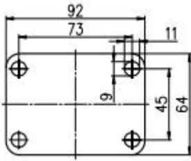
Plate Swivel
